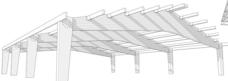
Charpente lamellé-collé
